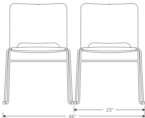
Armless Ganging Dimensions
